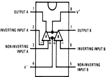
DIP/SO Package (Top View)
